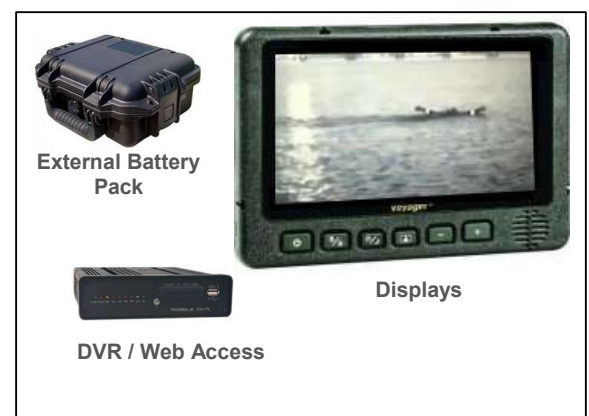
TugCam Ecosystem
